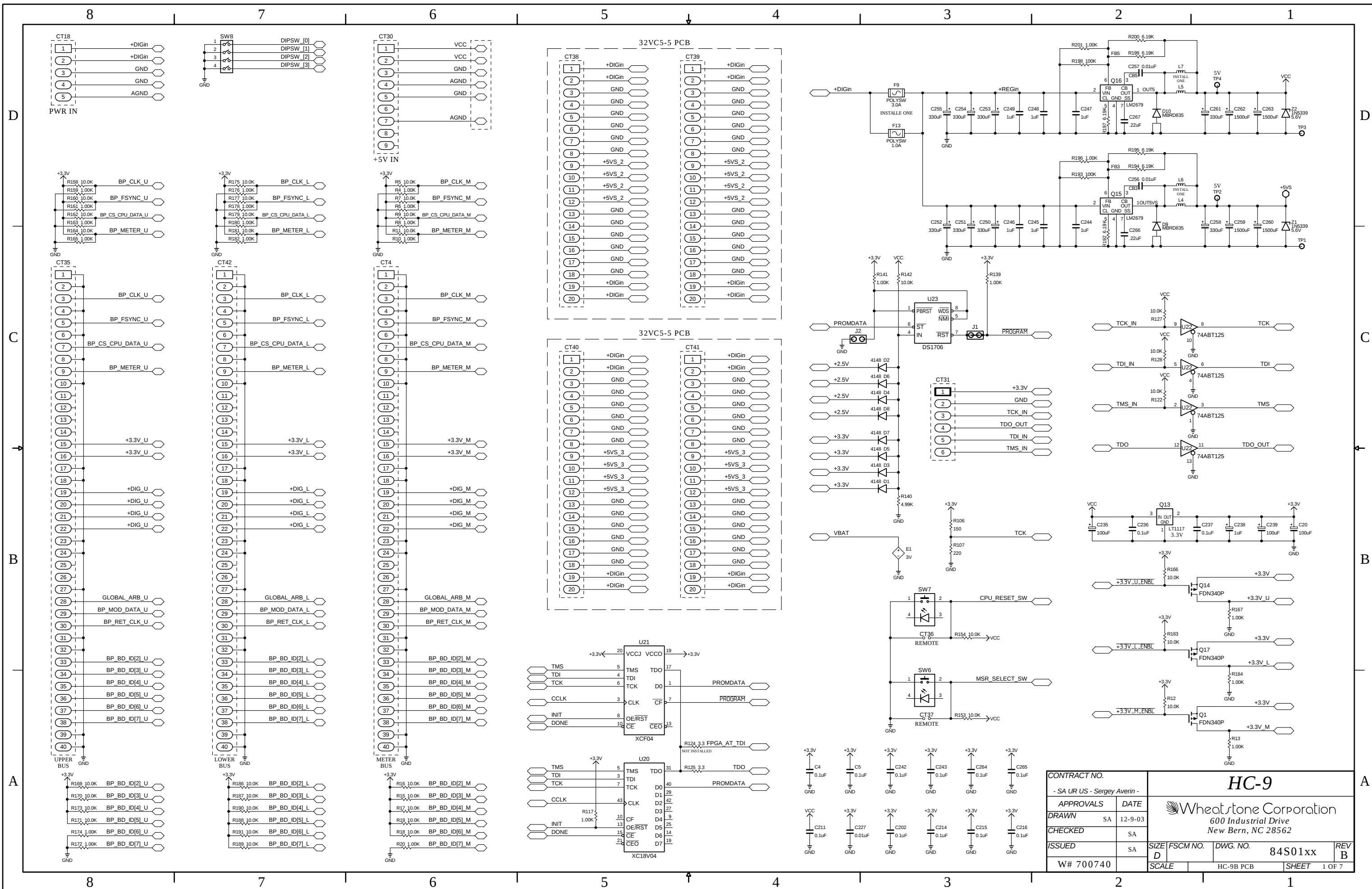
HC-9 Host Controller Module Schematic - Sheet 1 of 7
